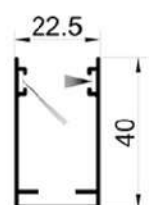
Guia Antiviento Coulisse Anti-Vent Guide Against wind
